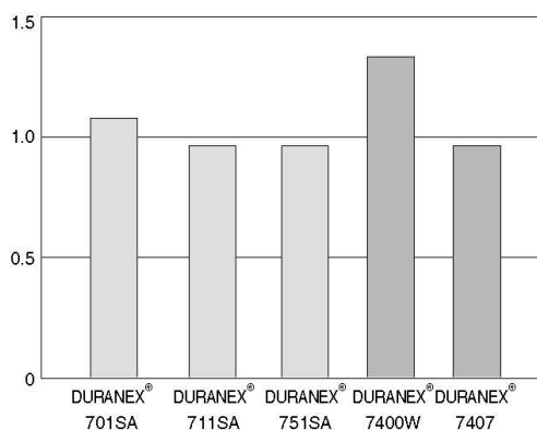
Figure 1-2 Internal warpage in molded box
